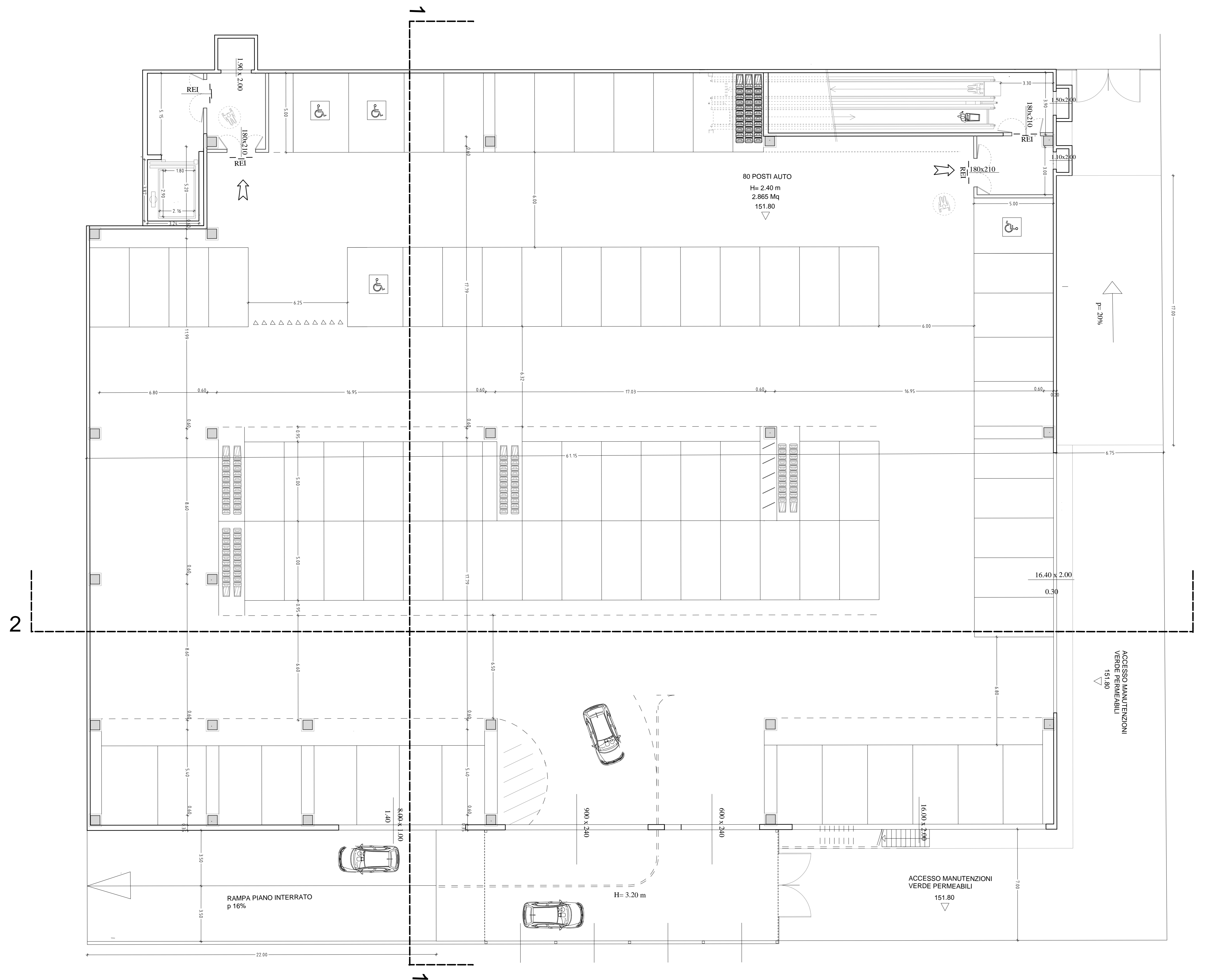
PIANO INTERRATO
